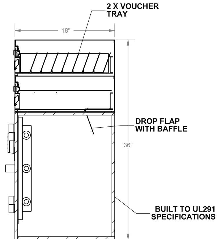
SIDE SECTION
