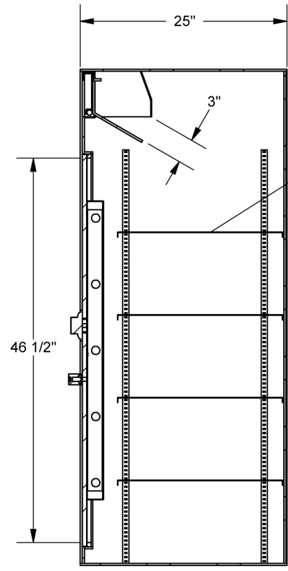
SIDE SECTION
